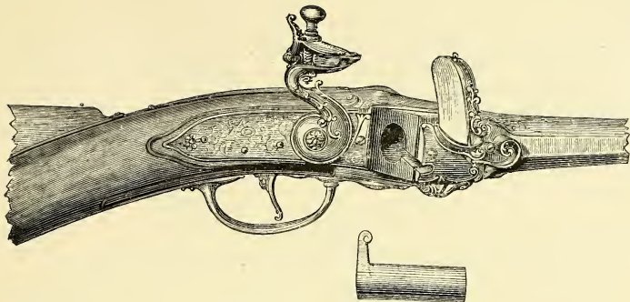
Italian Flint-lock Breech-loader.
